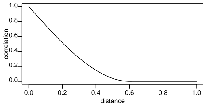
FIGURE 1.6. The spherical correlation function with \phi = 0.6 .
