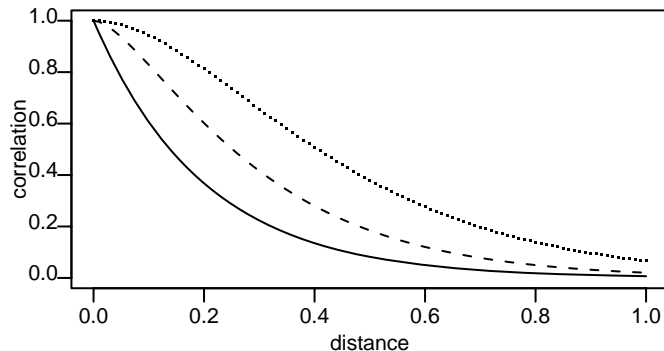
FIGURE 1.4. The Matérn correlation function with \phi = 0.2 and \kappa = 1 (solid line), \kappa = 1.5 (dashed line) and \kappa = 2 (dotted line).
