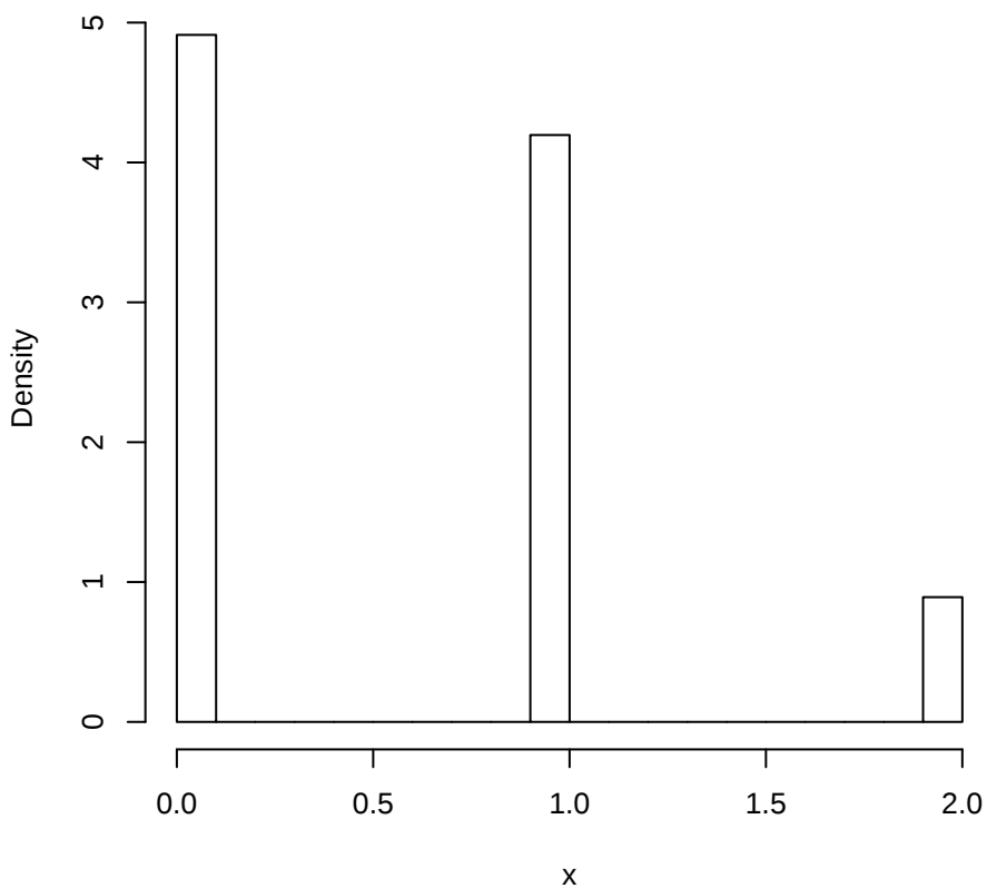
histogram of B(2,0.3)
