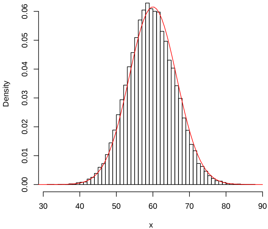
histogram of B(200,0.3)
