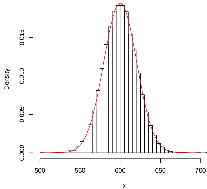
histogram of B(2000,0.3)
