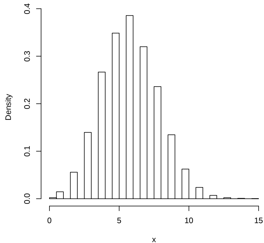
histogram of B(20,0.3)
