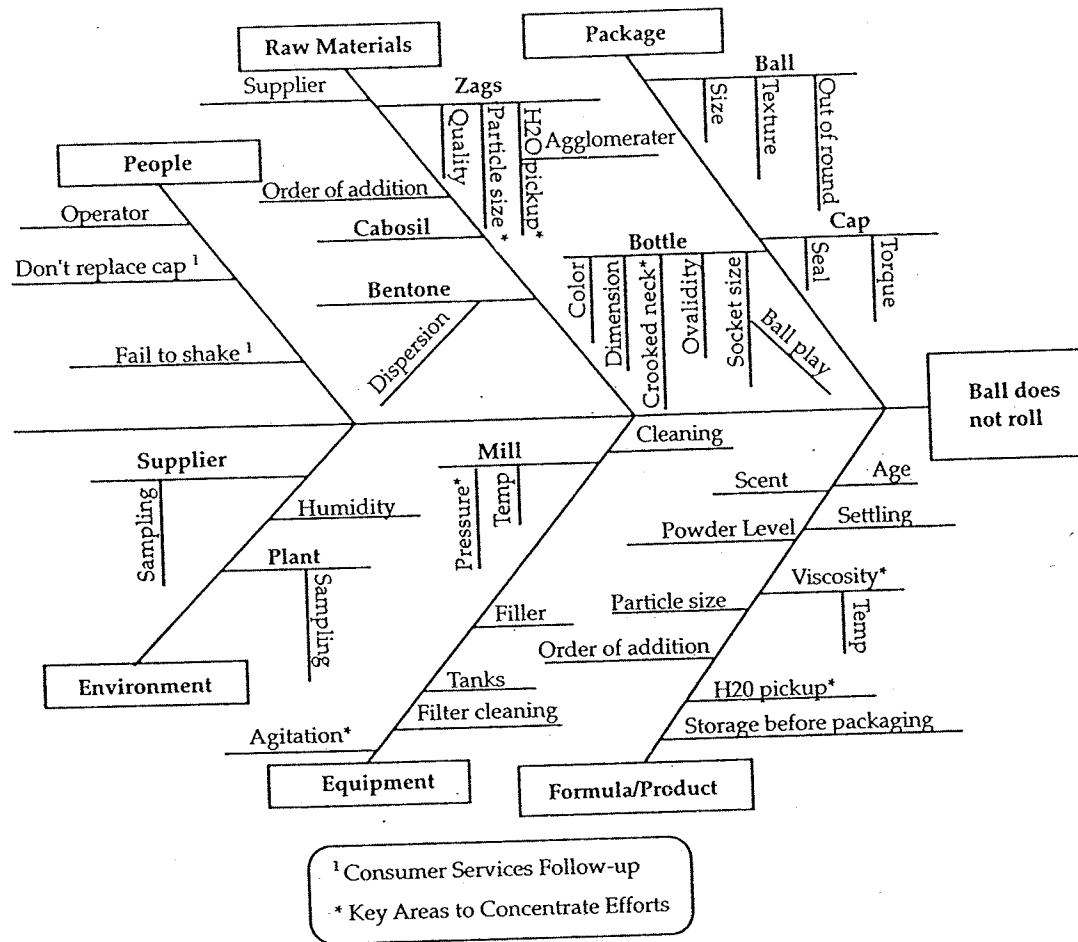
FIGURE 2.14 Cause and Effect Diagram for Factors Affecting the Ball Not Rolling in Assembled Deodorant Bottles
