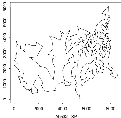
Figure 2: The best tour found by dynamic weighting for a 532-city TSP. The tour length is 27744 compared to the exact minimum of 27686. (Wong and Liang, 1997)
