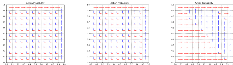
Figure 4: Mean policy probabilities for the indoor escape environment: (a) known optimal solution; (b) learned by LKTD; (c) learned by DQN, failing to explore different policies.
