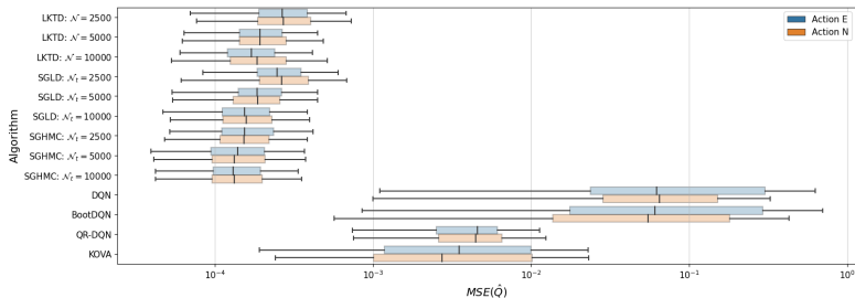
Figure 2: Boxplots for MSE(\hat{Q}_a) (for a \in \{N, E\} )
