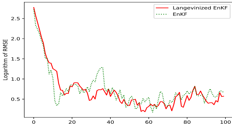
Figure: State estimates produced by LEnKF (red) and EnKF (green) for the Lorenz-96 model: \log(\text{RMSE}_t) along with stage t .
