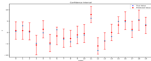
Figure 2: Prediction intervals of 20 testing points, where y-axis is for response, x-axis is for index of test points, and the blue point represents the true observation.
