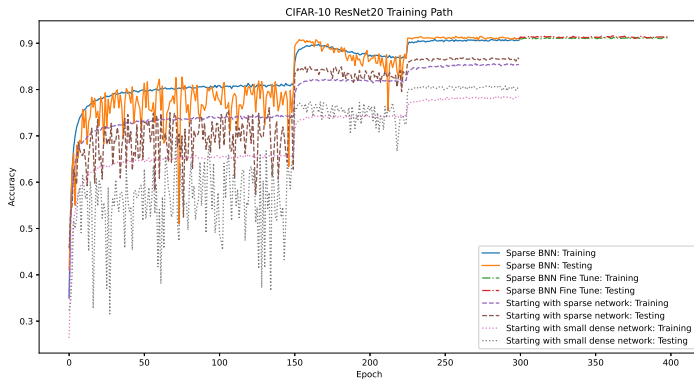
Figure 3: Training and testing paths of a ResNet20 model (with 10% sparsity level) on the CIFAR-10 dataset.
