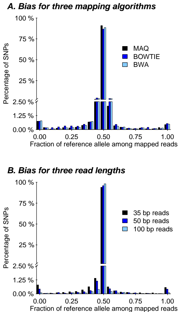
Fig. 4. Bias for three short-read alignment programs and for three read lengths. (A) The plot shows the distribution of the fraction of mapped reads that carry the reference allele. Simulated reads with an error rate of 0.01 were mapped to the masked genome using MAQ (black), BOWTIE (dark blue), and BWA (light blue). Other details as in Figure 2B. (B) As in A except reads contained no additional errors and read lengths were as indicated.
