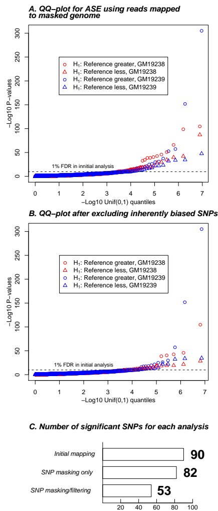
Fig. 5. Summary of the ASE results after SNP masking, and after excluding inherently biased SNPs. (A) Distribution of ASE P-values after masking known SNP variation. Masking has largely eliminated bias toward the reference allele (circles: over-representation of reference allele; triangles, over-representation of non-reference allele), however, the number of significant results is not reduced. Display is as in Figure 1B. The horizontal dashed line represents the P-value threshold of P = 5.5 \times 10^{-5} that allowed an FDR of 1% in the analysis presented in Figure 1. The FDR for this analysis using the initial P-value threshold was also 1%. (B) Distribution of P-values after excluding SNPs with an inherent bias toward one allele, as determined by simulations of perfect reads. This set of significant results is likely much more reflective of genes that show genuine allele-specific expression. The FDR for this analysis using the initial P-value threshold here was 1.4%. (C) Barplot showing the number of significant results for the three read-mapping strategies used in this paper, corresponding to Figures 1B, 5A and 5B, using a P-value cutoff of P = 5.5 \times 10^{-5} , corresponding to FDRs of 1.0%, 1.0%, and 1.4%, respectively
