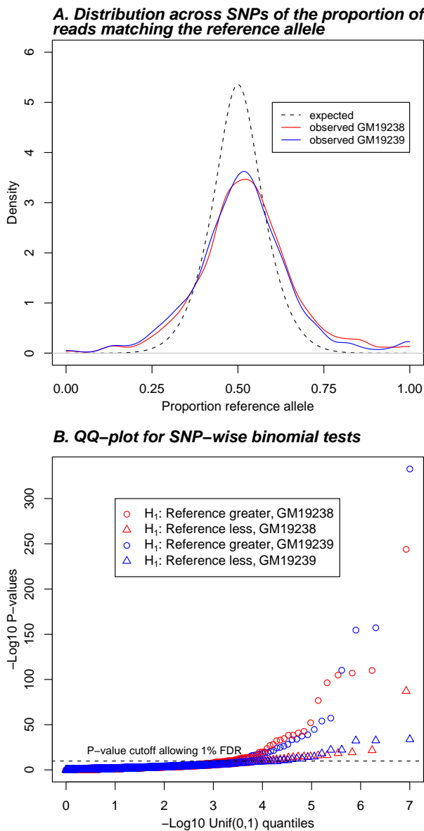
Fig. 1. RNA-Seq data show a higher variance in the relative expression of each allele and a skew toward high expression of the reference allele compared to the predicted distribution. (A) Estimated probability densities for the proportion of reads matching the reference allele (i.e., the allele given in the reference human genome sequence) at heterozygous SNPs in exons. Solid lines correspond to the observed distributions for known heterozygous SNPs with more than 20 reads in two Yoruba HapMap individuals. The dashed line shows the predicted distribution without reference bias or ASE. (B) QQ-plots of P-values for one-sided tests that expression of the reference allele is either higher (circles) or lower (triangles) than the non-reference allele. The horizontal dashed line is the P-value threshold corresponding to a false discovery rate of 1.0%. Notice the enrichment of very significant P-values for over-expression of reference alleles.
