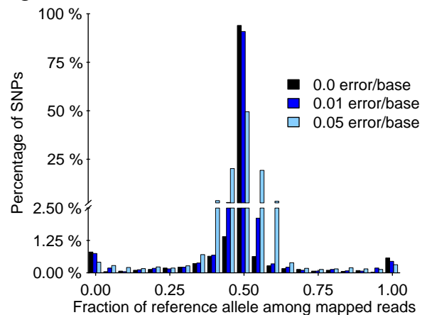
Fig. 2. Magnitude of read-mapping biases in simulated data. (A) The distribution (across SNPs) of the proportion of correctly mapped reads that carry the reference allele, compared to the non-reference allele. The y-axis is broken into two segments to show more clearly the rates of highly biased SNPs. Three different rates of sequencing errors are shown. (B) Read-mapping was performed as in (A), except that the reads were aligned against a version of the genome sequence in which all SNP locations were masked. Notice that for both analysis methods, some SNPs are strongly biased, and that SNP masking does not clearly improve the results. Sequencing errors can substantially increase the extent of bias.
