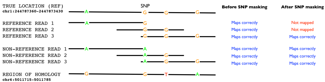
Fig. 3. Two examples in which homology with other genomic locations leads to read-mapping biases. Each example shows the variable sites in: (top row) the reference version of the genome sequence in the true location; (next six rows) three sample reads carrying the reference and three sample reads carrying the non-reference alleles at the SNP, and (bottom row) the sequence in a region of homology elsewhere in the genome. The right-hand columns show how each read is mapped with, and without SNP masking. In these examples a read is mapped to a particular location if it has a unique best match at that location, and is unmapped if there is a tie between possible locations. The SNP masking generates a 1-nucleotide mismatch between both alleles and the reference sequence at the masked site.
