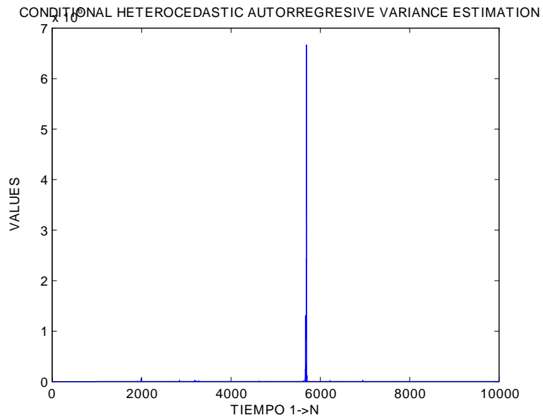
Fig. 2. Variance estimation for the above time series
