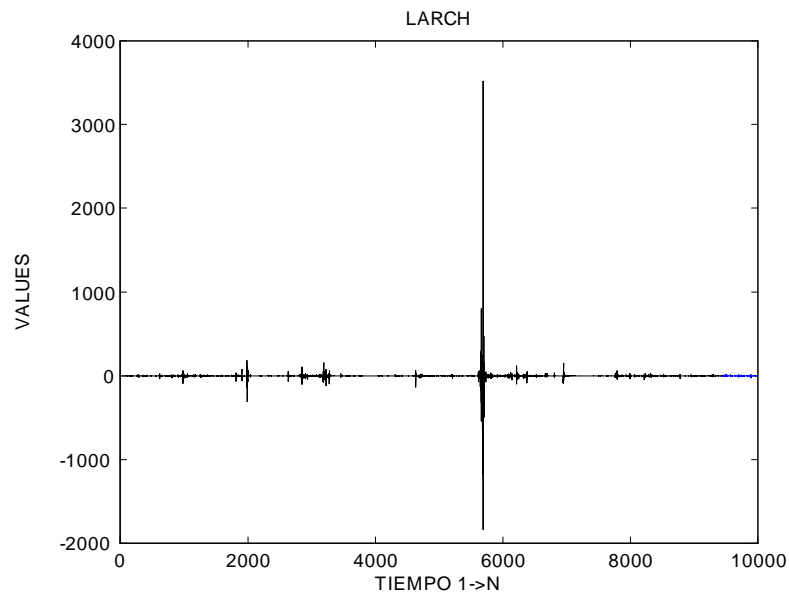
Fig. 1. Observation values for a typical LARCH time series
